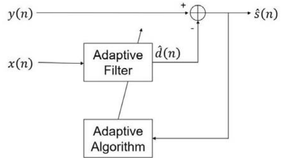
Fig. 2 Internal structure diagram of the AEC
